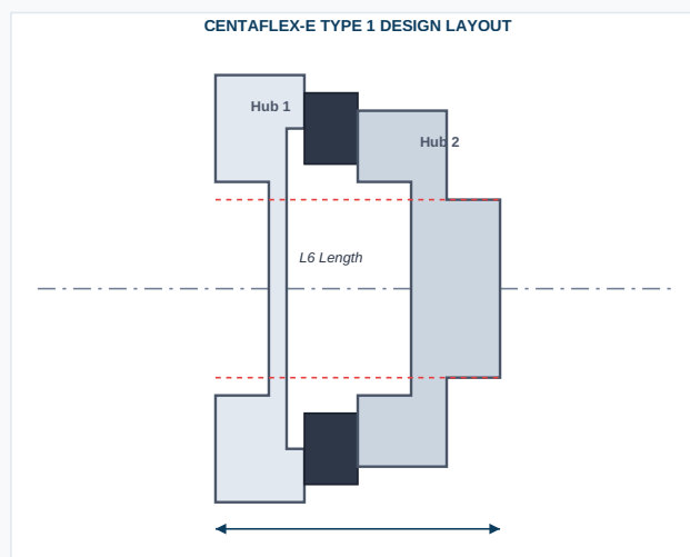
Figure 1: Sectional structural layout blueprint detailing Hub 1, Hub 2, and intermediate elastomeric shock absorbers for CENTAFLEX-E Bauform 1.
